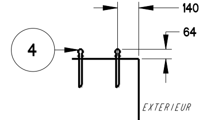
DETAIL B SCALE 1/25
