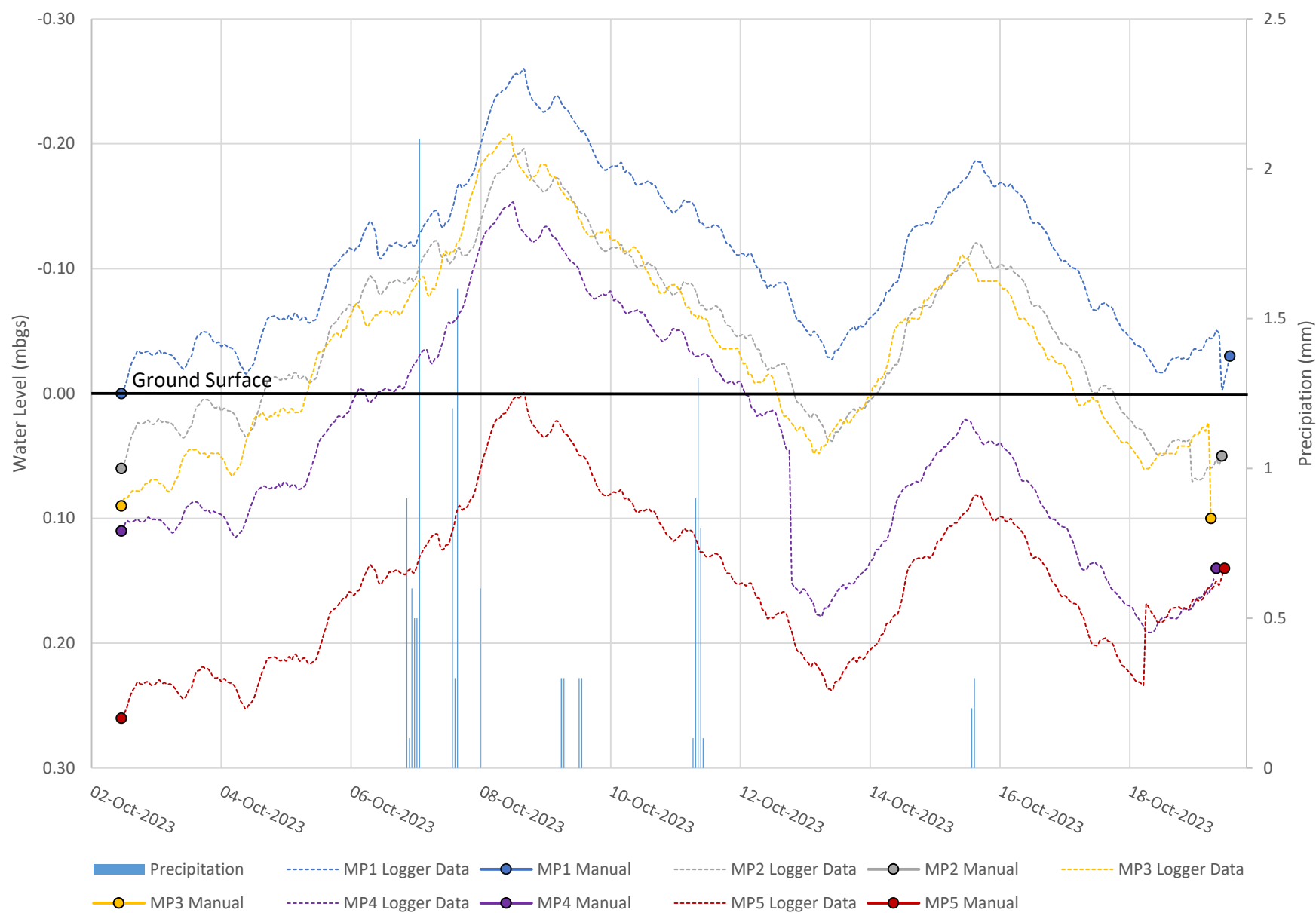
Figure 11. BBR Mini-Piezometer Hydrograph
